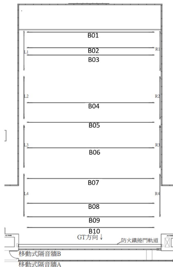
Figure showing the position of the fly bars and the movable sound insulating wall B
