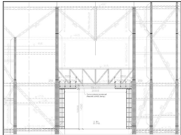
GT Maximum Proscenium Opening(in cm)
